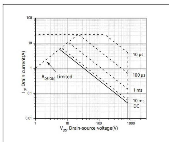
Fig12.Safe Operating Area
