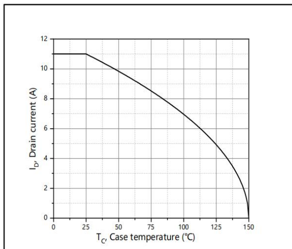
Fig8.IDS vs TC
