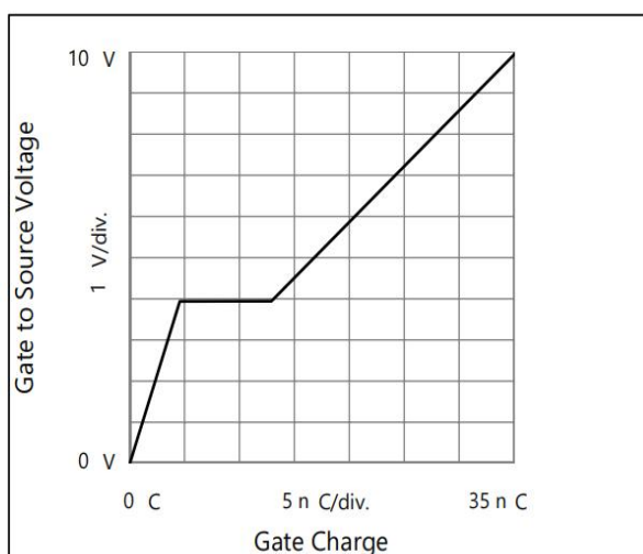
Fig10.Gate Charge Characteristics
